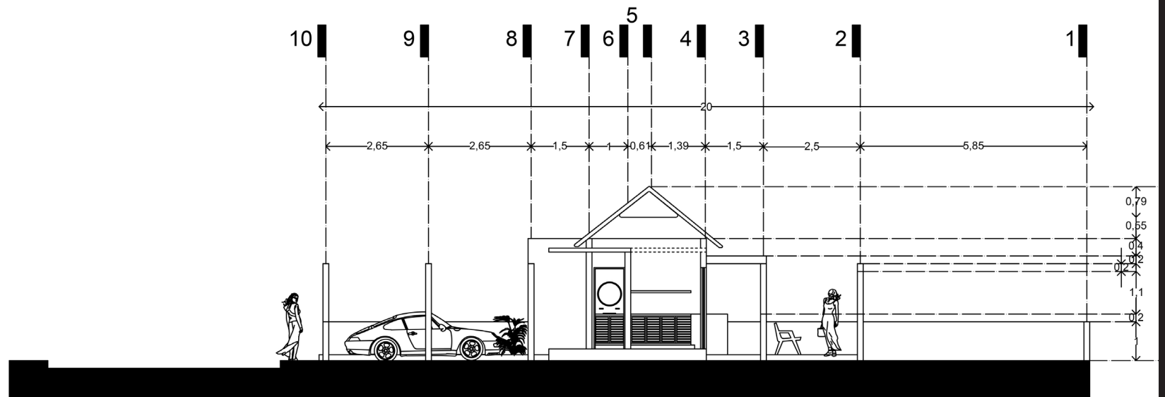
CORTE y1-y1
